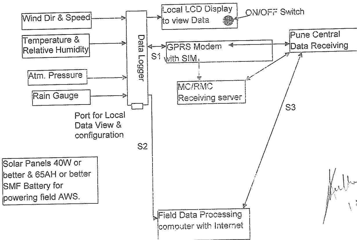
Basic Block Diagram of Field site AWS and its Communication
